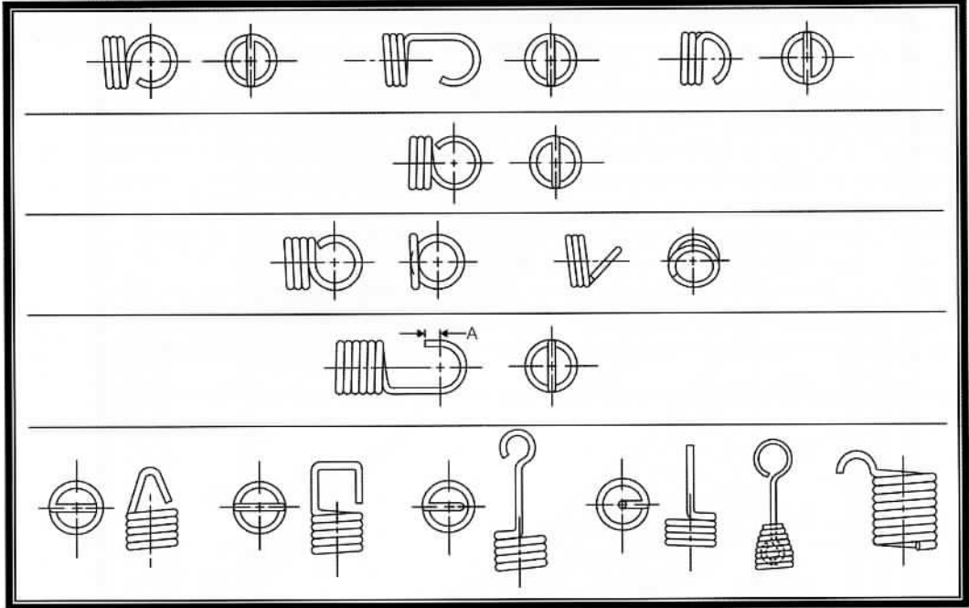
Figure 36. Common End Configurations for Helical Extension Springs.
